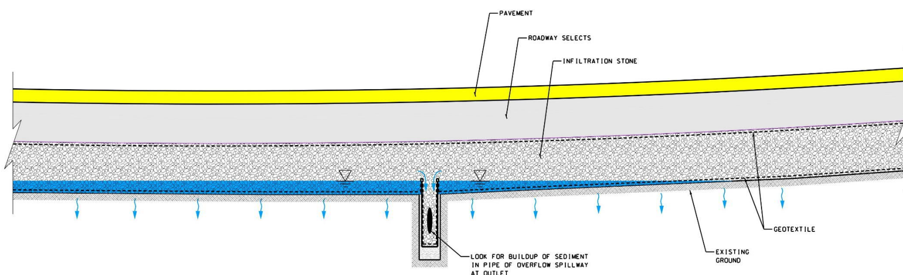
WALPOLE - CHARLESTOWN 14747 INFILTRATION BMP DIAGRAM LONGITUDINAL SECTION
