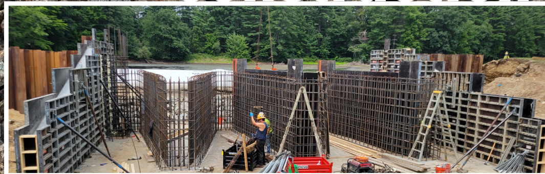
New 150-ft labyrinth weir in the footprint of 50-ft gravity weir
